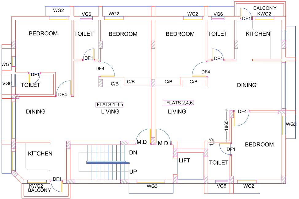
TYPICAL FLOOR PLAN(1,2,3)
